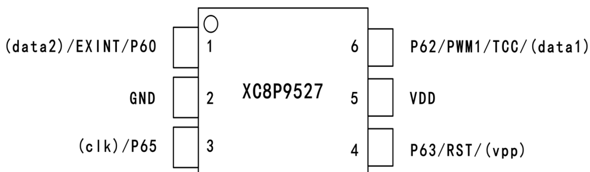
XC8P9527-6PIN 脚位图
