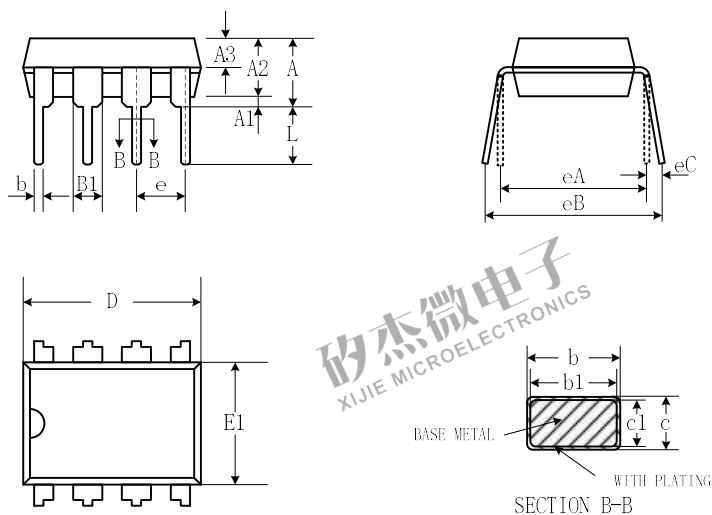
DIP8
