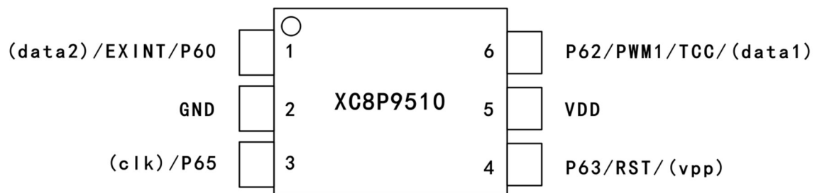
XC8P9510-6PIN 脚位图
